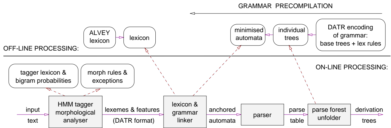
Figure 1: System architecture
