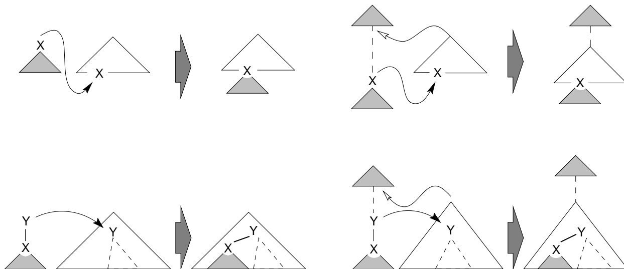
Figure 2: Composition operations
