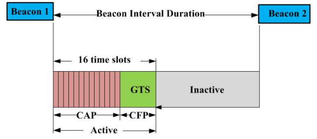
Fig. 3: Superframe Structure [48]
