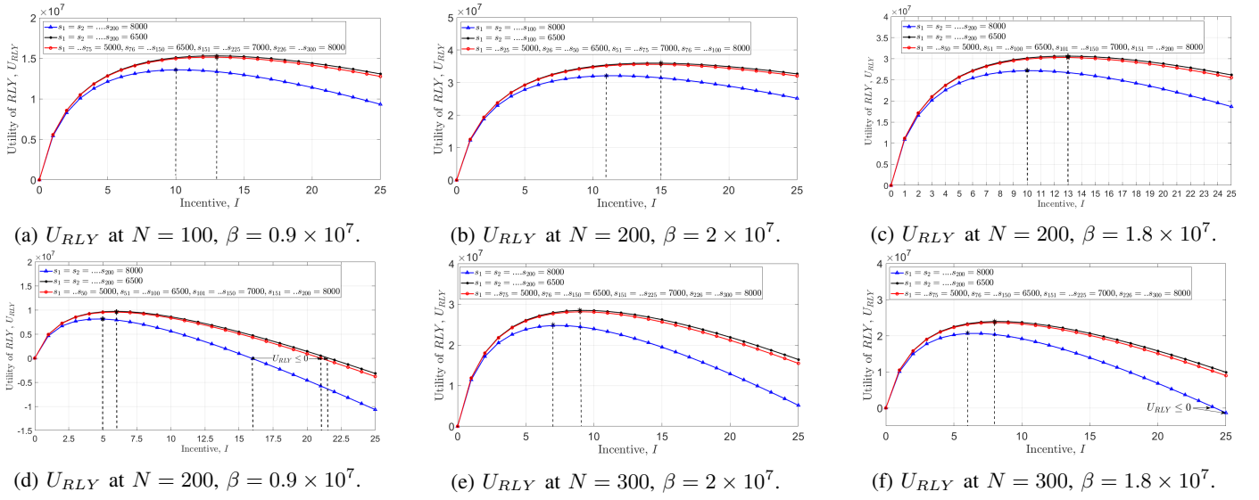
Fig. 11: U_{RLY} with equilibrium points (*) of Stackelberg Game.
