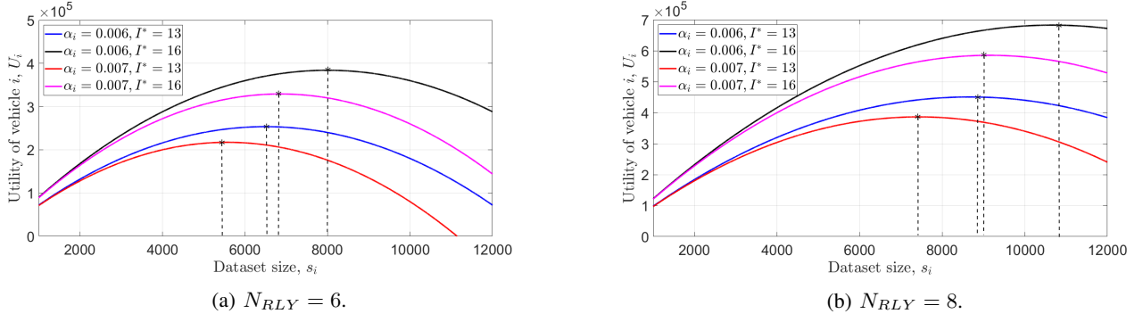
Fig. 10: U_i with equilibrium points (*) of Stackelberg Game.
