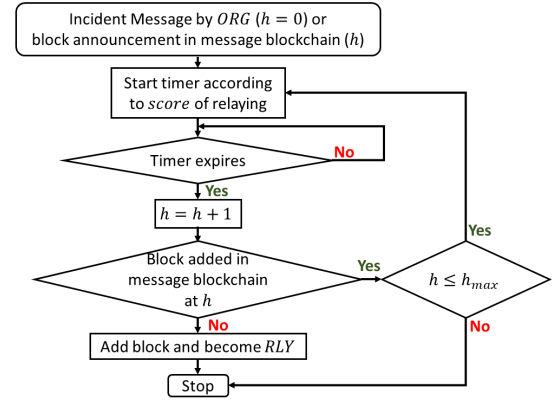
Fig. 4: Flowchart of actions by vehicle i according to PoFL based Message Dissemination.
