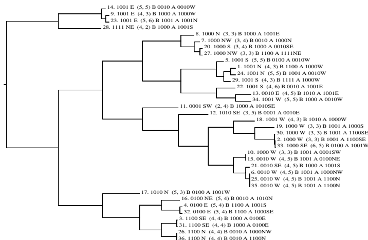
Figure 6: Cluster analysis of all location codes used in the DISOS route. Labels indicate the move number that produced the code, the description vector for the location, the move made, the coordinates of the location, the description vector of the previous place, the description vector of the following place, and the move taken to get there.
