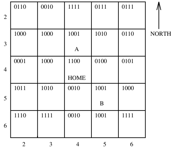
Figure 4: The region of the grid world used in the experiments. The four-bit binary vector at each location indicates the description or sensation vector associated with that location.
