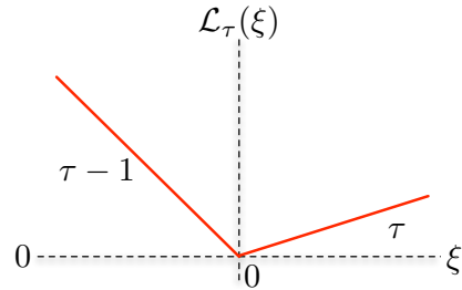
Figure 1. The pinball loss function.
