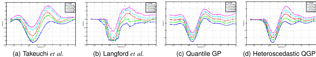
Figure 2. Illustration of conditional quantile analysis for Silverman’s motorcycle dataset via Quantile SVM (Takeuchi et al. ), Reduction (Langford et al. ), Quantile GP, and Heteroscedastic QGP. The dataset exhibits heteroscedasticity. Non-crossing constraint is not enforced in Reduction and enforceable in Quantile SVM via additional linear constraints and is an inherent property of Quantile GP.
