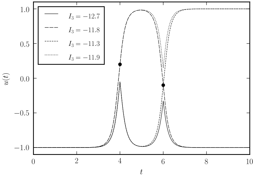
FIG. 6.1. Illustration of the problem of local minima of I for the smoothing problem with a small number of observations. The process u(t) starts at u(0) = -1 and moves in a double-well potential with stable equilibrium points at -1 and +1 . Two observations of the process are indicated by the two black circles. The curves correspond to four different local minima of the functional I_3 for this situation.
