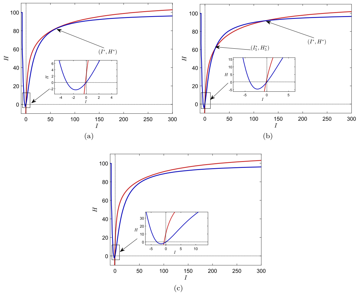
Fig. 4 (a–c) Intersection scenarios of isoclines (4) and (5) for R_0 < 1 . Blue curve depicts isocline (4) and red curve depicts isocline (5)
