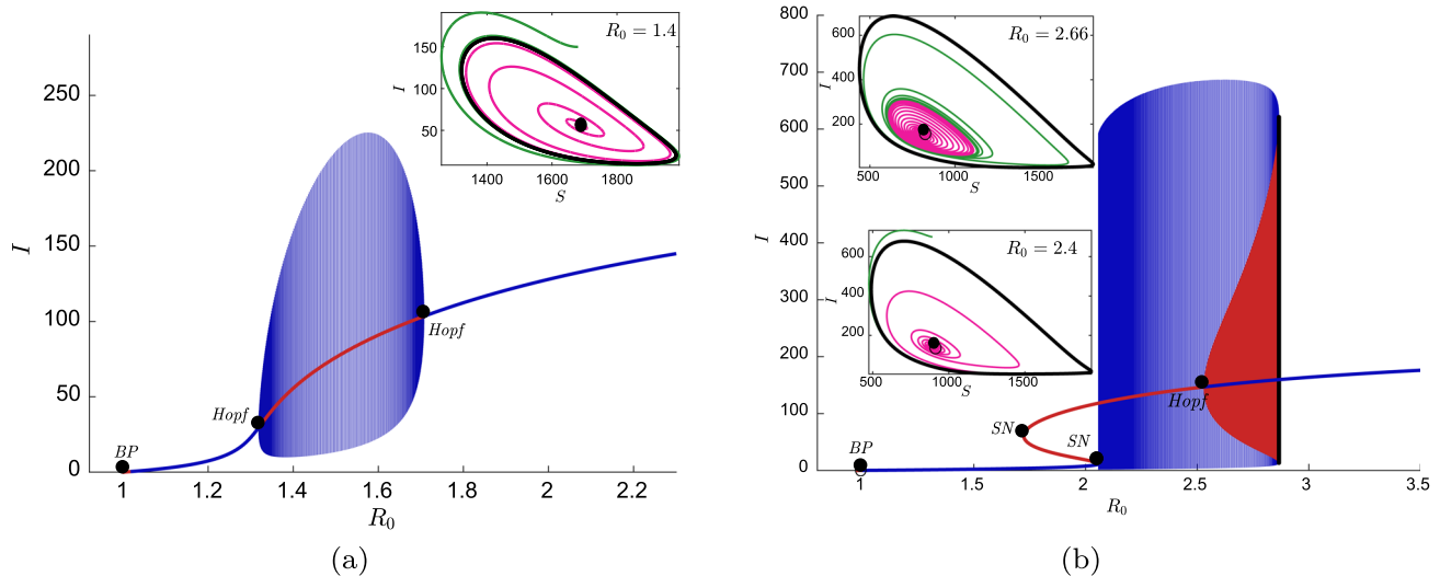
Fig. 6 Bifurcation plot in R_0 - I plane for a k_1 = 0.0008 b k_1 = 0.005
