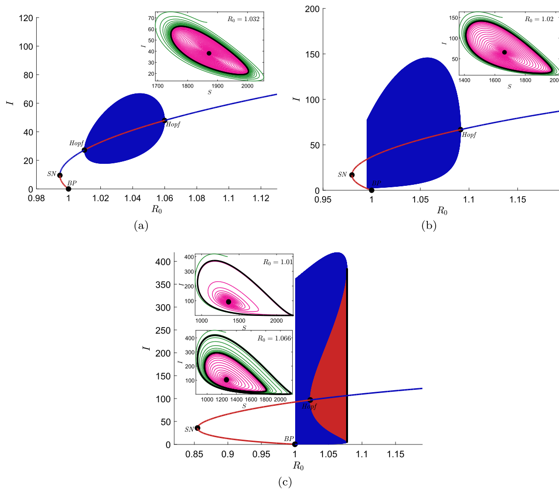
Fig. 9 Bifurcation plot in R_0 - I plane for a k_0 = 0.00122 b k_0 = 0.0014 (c) k_0 = 0.0024
