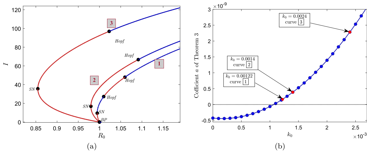
Fig. 8 a Equilibrium curves in R_0 - I plane for k_0 = 0.00122 (labeled as [1]), k_0 = 0.0014 (labeled as [2]) and k_0 = 0.0024 (labeled as [3]) b Plot for coefficient a of Theorem 3 with respect to k_0
