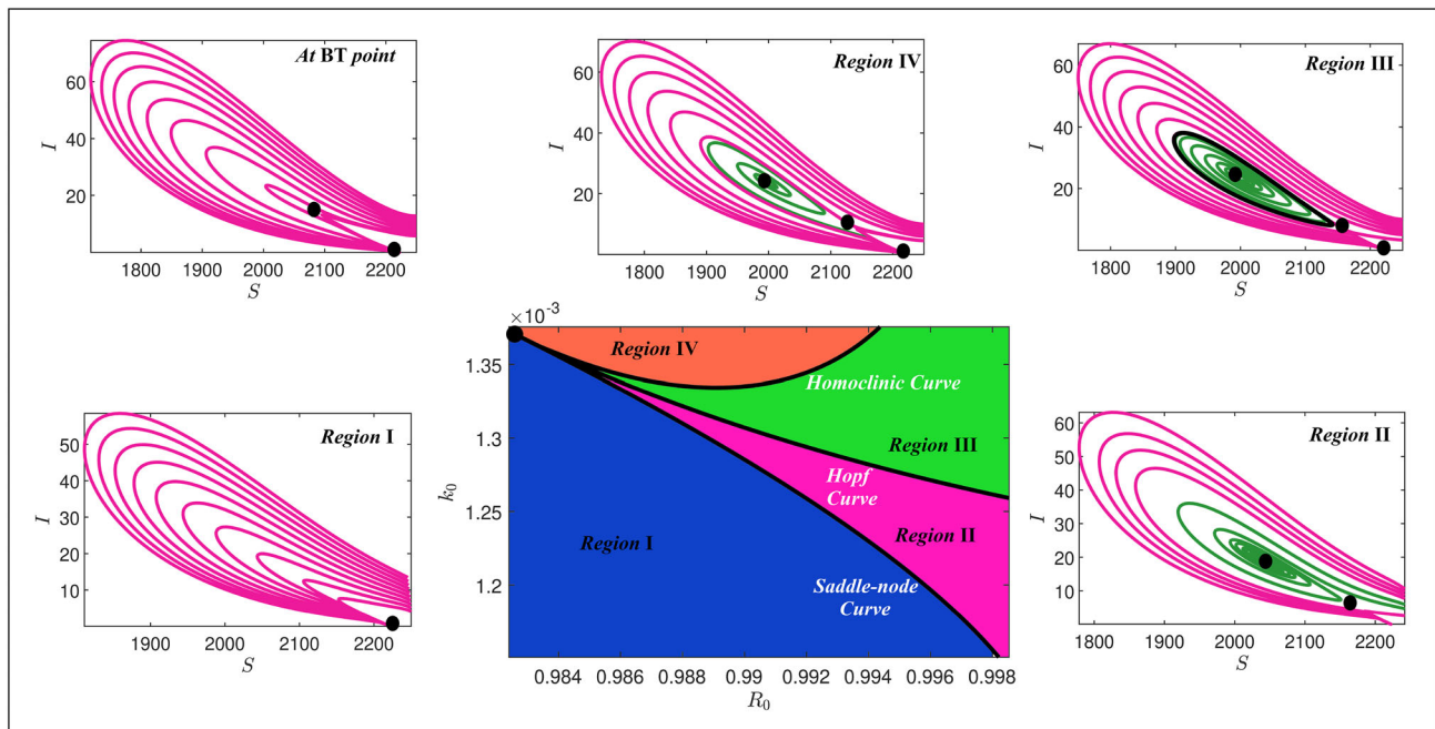
Fig. 10 Unfolding of BT point in R_0 - k_0 plane and phase portraits at BT point and corresponding to Region I, II, III, and IV. In Region I, model system (1) only has a stable disease-free equilibrium. In Region II, there are two unstable endemic equilibria. In Region III, there are two unstable endemic equilibria, and a stable limit cycle surrounds the endemic equilibrium with high endemicity. In Region IV, there are two endemic equilibria, one stable and the other unstable
