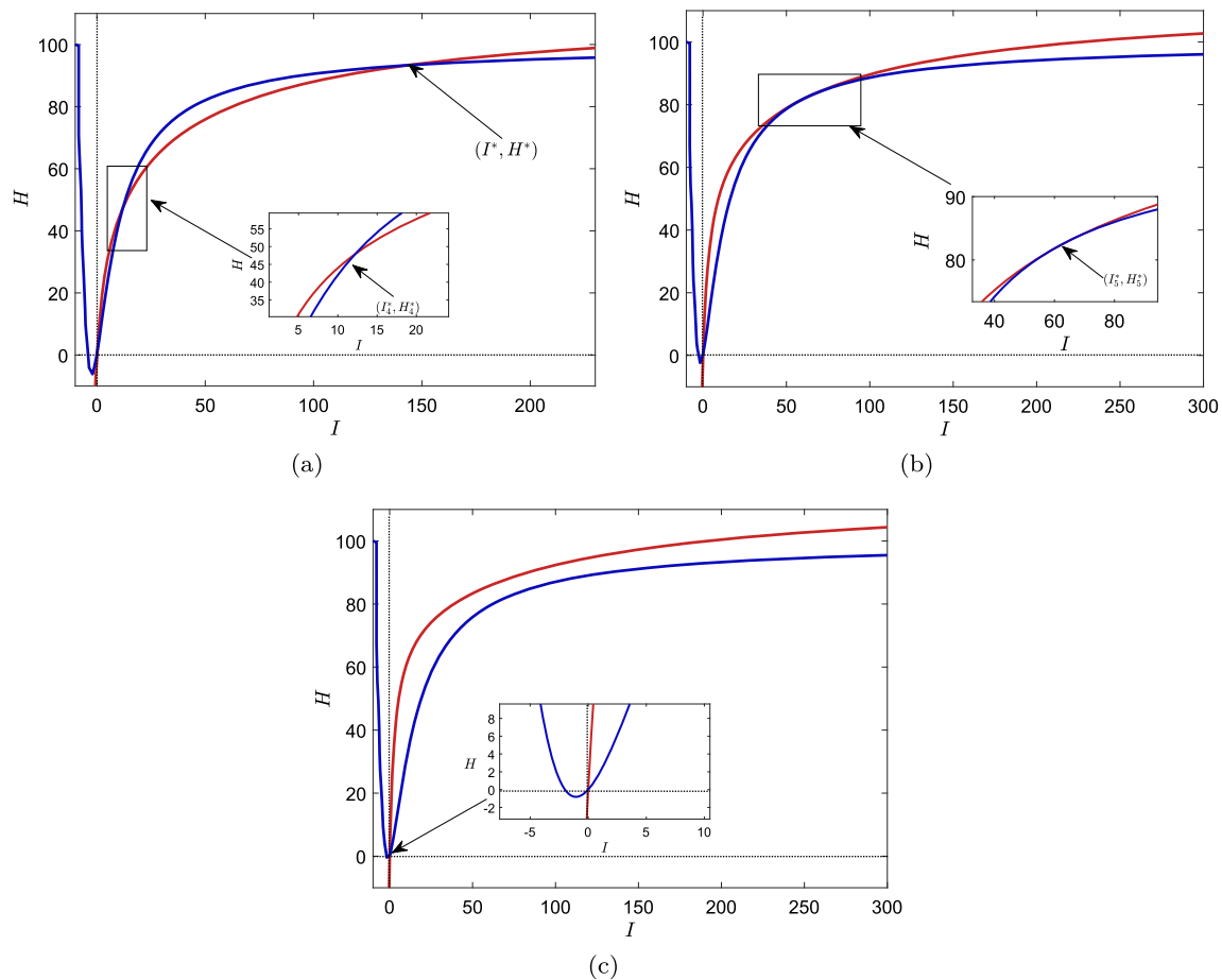
Fig. 3 (a–c) Intersection scenarios of isoclines (4) and (5) for R_0 = 1 . Blue curve depicts isocline (4) and red curve depicts isocline (5)
