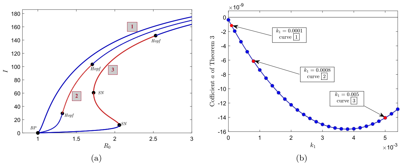
Fig. 5 Equilibrium curves in R_0 - I plane for k_1 = 0.0001 (labeled as 1), k_1 = 0.0008 (labeled as 2) and k_1 = 0.005 (labeled as 3)
