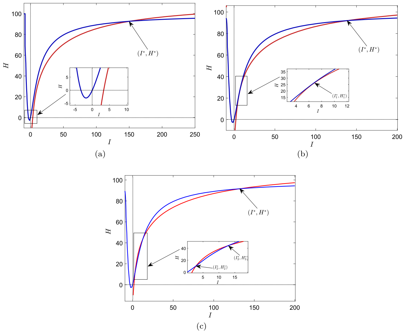
Fig. 2 (a–c) Intersection scenarios of isoclines (4) and (5) for R_0 > 1 . Blue curve depicts isocline (4) and red curve depicts isocline (5)
