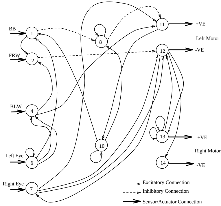
Fig. 6. The same C1 network as in the previous figure, but with redundant and non-visual units deleted.
