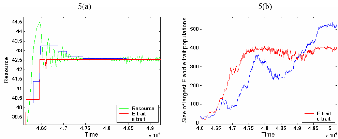
Figure 5: Close up view of the establishment of regulation during a typical simulation run. Figure (a) shows the resource levels to which the largest E and e allele subpopulations are adapted; figure (b) shows the size of these two subpopulations. Figure (a) shows the resource (green line) becoming regulated around the two subpopulations, with [E, A_{low}] and [e, A_{high}] visible in red and blue respectively. During the establishment of regulation, the size of the two subpopulations increases until the majority of the population belong to one of these two groups (figure b). Note that even after regulation is established there are continuous oscillations in the resource.
