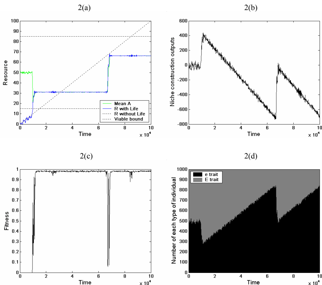
Figure 2: Typical run of the simulation with two periods of regulation. Figure (a) plots the resource over time (blue line); mean A is the mean resource level that the population is adapted to; the diagonal dotted line is the forcing target P ; the horizontal dotted lines are the bounds of viability outside of which life cannot survive. Figure (b) plots the total niche construction output of the population. Figure (c) plots the mean fitness of the population. Figure (d) is a stacked bar chart showing the number of individuals with the E allele (who increase the resource), and the number of individuals with the e allele (who decrease the resource).
