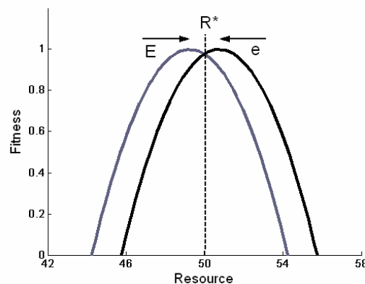
Figure 4: The fitness range of the [E, A_{low}] type is plotted with a solid grey line; the [e, A_{high}] type's fitness range is plotted with a solid black line. The vertical dashed black line marks the value for R^* . The resource will be maintained, on average, around this value. When R is closer to the [E, A_{low}] type, E alleles increase in frequency relative to e alleles, raising resource levels. Conversely, when R is closer to the [e, A_{high}] type, the relative fitness of the two types leads to the resource decreasing. The niche construction of each subpopulation pushes the resource towards R^* , thus counteracting the niche construction of the opposing subpopulation, and together regulating R against perturbations.
