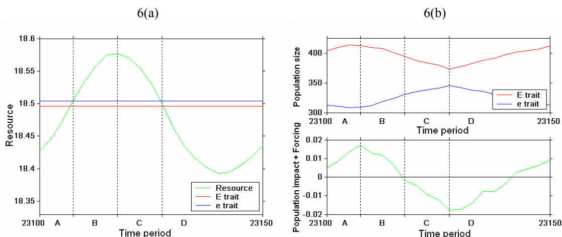
Figure 6: Close up view of a typical oscillation in the resource. The vertical dotted lines separate the oscillation into four time periods: A, B, C, D. Figure (a) shows the resource (green line), and the resources levels that [E, A_{low}] and [e, A_{high}] are adapted to (the red and blue lines respectively). Figure (b) shows the size of the [E, A_{low}] and [e, A_{high}] subpopulations. It also shows total effect that the population and forcing has on the resource at each time step (green line). When this is negative the net effect of the niche construction and forcing decreases the resource; when it is positive the resource will be increased.
