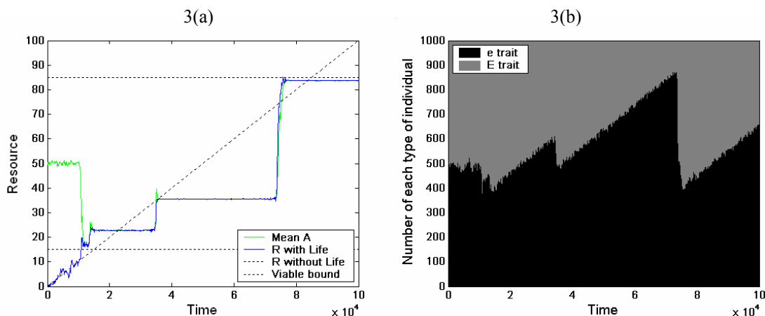
Figure 3: Typical run of the simulation with three periods of regulation. Figure (a) plots the resource over time (blue line); mean A is the mean resource level that the population is adapted to; the diagonal dotted line is the forcing target P ; the horizontal dotted lines are the bounds of habitability outside of which life cannot survive. Figure (b) is a stacked bar chart showing the number of individuals with the E allele (who increase the resource), and the number of individuals with the e allele (who decrease the resource).
