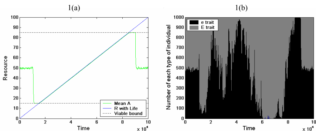
Figure 1: Typical simulation run with no niche construction effect. Figure (a) plots the resource over time (blue line); mean A is the mean resource level that the population is adapted to; the horizontal dotted lines are the bounds of habitability outside of which life cannot survive. Figure (b) is a stacked bar chart showing the number of individuals with the E allele and the number of individuals with the e allele.
