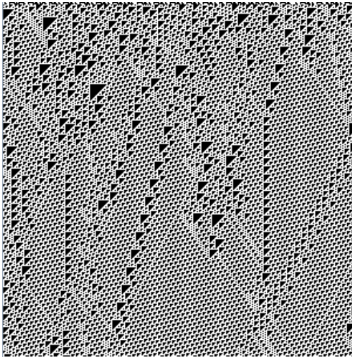
rule 137 (193 r )
