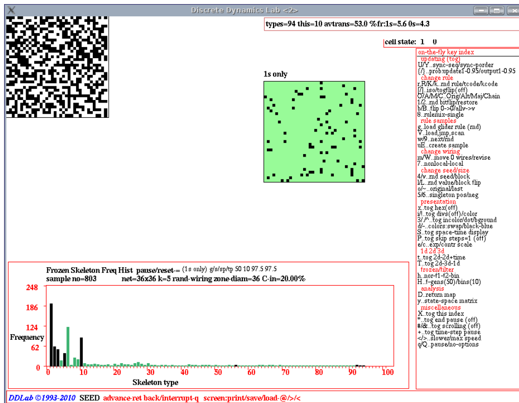
Figure 31.21: A snapshot of the DDLab screen, showing the skeleton histogram at sample 803 with 94 skeletons found.. The network is a 36 \times 36 v2k5 RBN with unbiased random wiring and 20% canalizing inputs (chapter 15). The parameters in section 31.8 (1s only), labelled g/s/sp/tp , are 50, 10, 97.5%, 97.5%. Each sample starts with a new random initial state, and the skeleton into which the transient falls is identified (if any). A skeleton that cannot be matched with a pre-existing type is added as a new type. The histogram columns are continuously updated (in black), showing the skeleton type ( x axis) against the frequency of arriving at that type ( y axis). The axes rescale automatically (and columns turn green) on reaching the current scale limits. Top left : a snapshot of the space-time pattern. Top center : the skeleton, pattern of frozen 1s. Bottom : the unsorted histogram.
