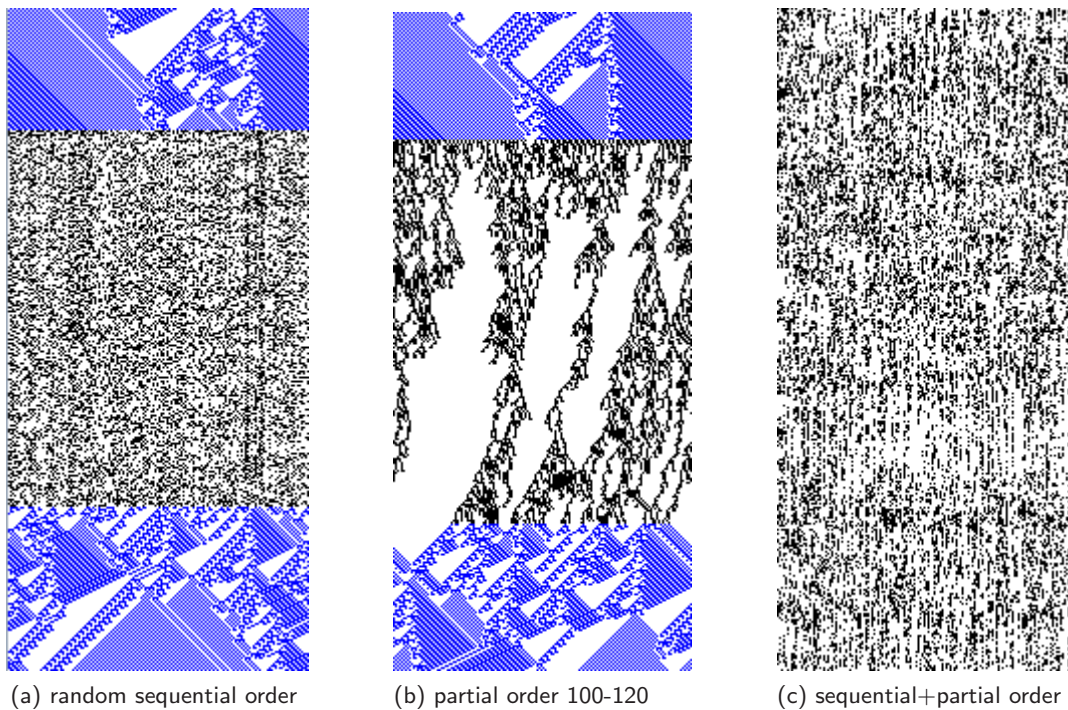
Figure 31.7: Examples of updating with sequential, partial order, and both orders combined, for a 1d CA v2k5 rcode(hex)bc82271c, n=150 . In case (a) and (b) parallel updating was switched to the new order on-the-fly, for about 180 time-steps, then back to parallel. In case (c) about 310 time-steps are shown with combined sequential and partial order updating
