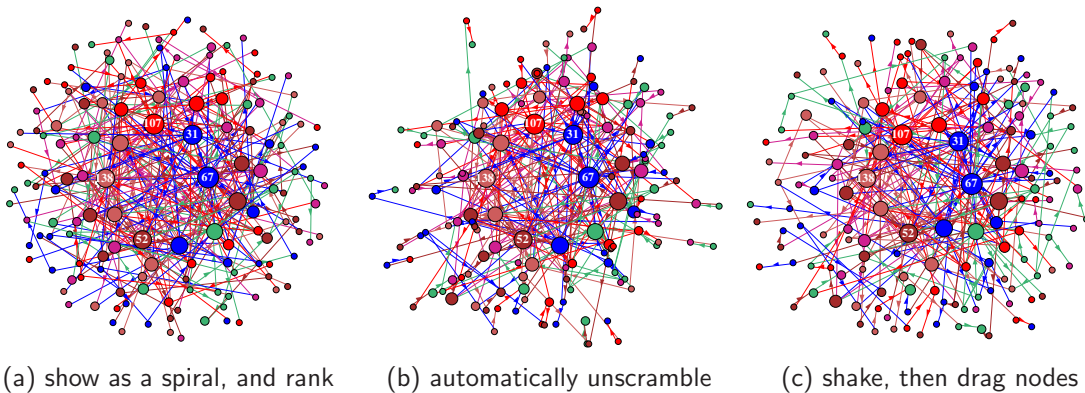
Figure 20.6: One possible method of unscrambling the network-graph of a scale-free RBN, n=150 .
