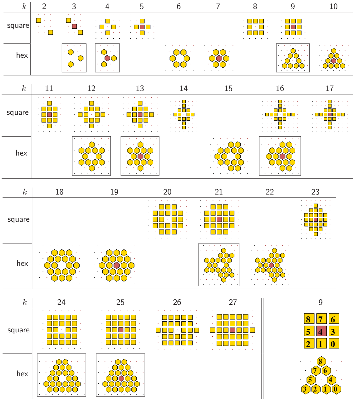
Figure 10.2: 2d neighborhood templates as defined in DDLab, for k=2 to 27, square, hex or both, designed for best symmetry. The target cell may be excluded and is otherwise shown red.
