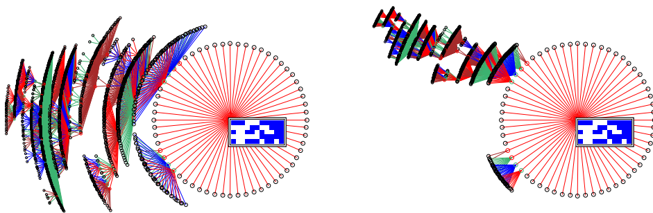
Figure 26.14: Decreasing the pre-image fan-angle of a subtree of a 1d CA v2k3 rcode(dec)110, n=55 . The subtree root, (hex)71f0cf34c0fcd, is highlighted as a bit pattern. Other nodes are show as spots. Left : default fan-angle (factor=1). Right : reduced fan-angle (factor=0.3). Note that the fan converging on the root of a subtree is always 360^\circ , and is not affected.
