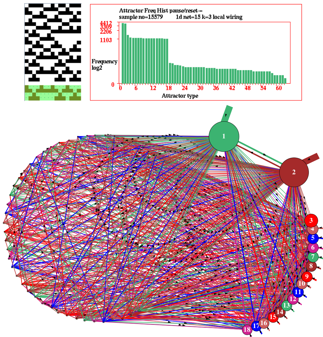
Figure 31.20: The attractor histogram jump-graph, for a 1d CA, v3k3 rcode(dec)54, n=15 . Top left : a sample space-time pattern showing the attractor repeated. Top Right : The attractor histogram with log y -axis, all 63 attractors were found after a sample of 15579. Above : the jump-graph (chapter 20.3) — nodes and links scaled according to attractor frequency which reflects basin volume, and the graph rearranged 20.5 starting from a circle layout.
