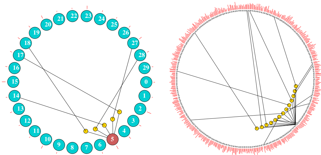
Figure 17.3: Examples of the 1d circle wiring graphic. Left: the same network as in figure 17.2, k=5 , n=30 . Right: k=13 , n=500 . The “active” cell is repositioned by mouse pointer clicks or moved by the arrow keys. Each cell’s “outwires” are represented by the length of the red radial lines outside the circle. The cell index is shown for networks smaller than about n=40 . For networks greater than about n=162 , the nodes themselves are not shown, but just the radial lines.
