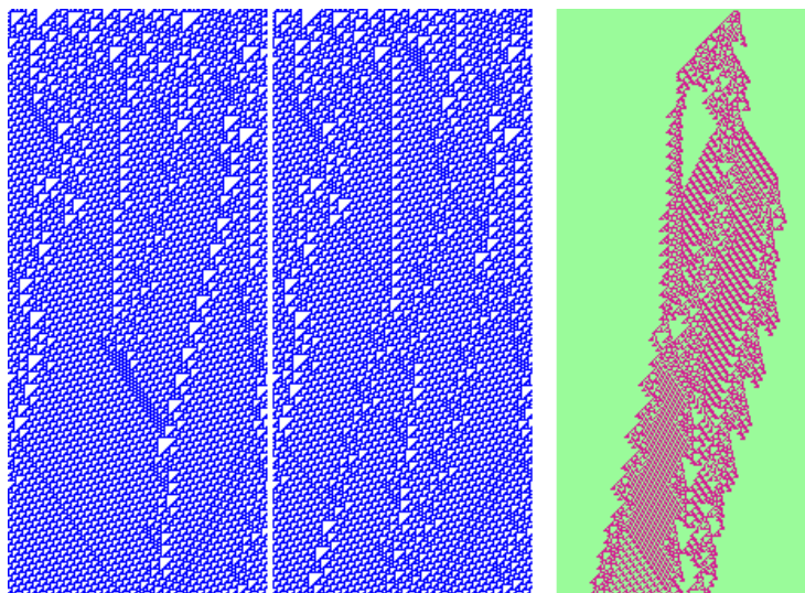
Figure 31.9: The difference in the dynamics between two 1d CA. Left: the space-time patterns of two identical CA (color by value), except that the random initial state differs by one bit. Right: the instantaneous difference between the two at each time-step shown as a third space-time pattern. v2k3 rcode (dec)110, n=150+150 .
