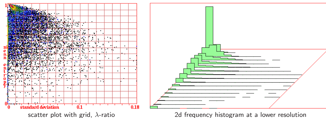
Figure 33.12: Left : The rule sample scatter plot — the same as in figure 33.10, but with a 16×16 superimposed grid — by entering grid-g in section 33.6.3. Right : The 2d frequency histogram of the rule sample scatter plot in figure 33.10 redrawn at a lower resolution, 16×16, selected in subdiv in section 33.6.3. The vertical axis is the frequency of rules falling on each square of the grid. This figure also illustrates pausing after each row with step-s or show%-S in section 33.6.3.
