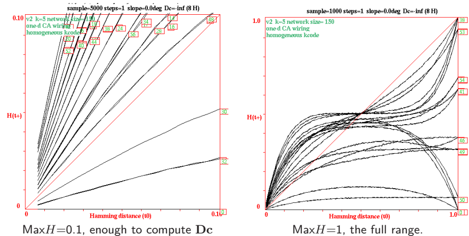
Figure 22.4: Analogous plots to figure 22.3 of the 64 v2k5 tcodes. The terminal printout will be just #: s n Dc because atcode and kcode rules are symmetric, so reflections reproduce the same rule. Above Left : for 36 equivalence classes, MaxH=0.1, enough to compute Dc (Dc sample=8H). Above Right : for 20 rule clusters, for the full range of Hamming distance
