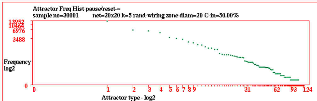
Figure 31.17: The attractor frequency histogram, for a 20 \times 20 RBN, v2k5 , with unbiased random wiring, and canalizing inputs set to 50% (chapter 15). Each sample starts with a new unbiased random initial state, and the attractor type into which the transient falls is identified, either as an existing type, or a new type which is added to the list of existing types. The histogram columns are continuously updated, in black, showing the attractor type ( x -axis) against the frequency of arriving at that type ( y -axis). Given a large enough sample, bar height indicates the relative size of the basin of attraction. The axes rescale automatically on reaching the current scale limits. Columns turn green when rescaled, redrawn, or sorted.
