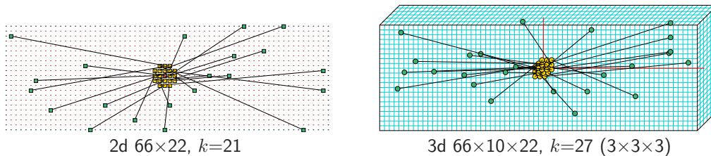
Figure 17.21: For homogeneous- k , enter rnd-R for totally unbiased random wiring, ignoring any biases set in section 17.9.6. The examples show wiring to the psuedo-neighborhood.
