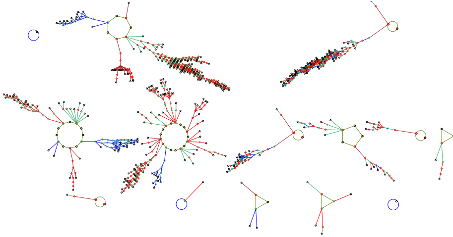
Figure 26.1: A basin of attraction field of a 1d CA with null boundary conditions (NBC) v2k3 rcode(dec)110 , n=10 . Compression does not apply with NBC, and the basins are very different from the same network with periodic boundary conditions (and no compression) in figure 26.4. In this example the basins were positioned within suitably rearranged jump-graph nodes (section 20.7).
