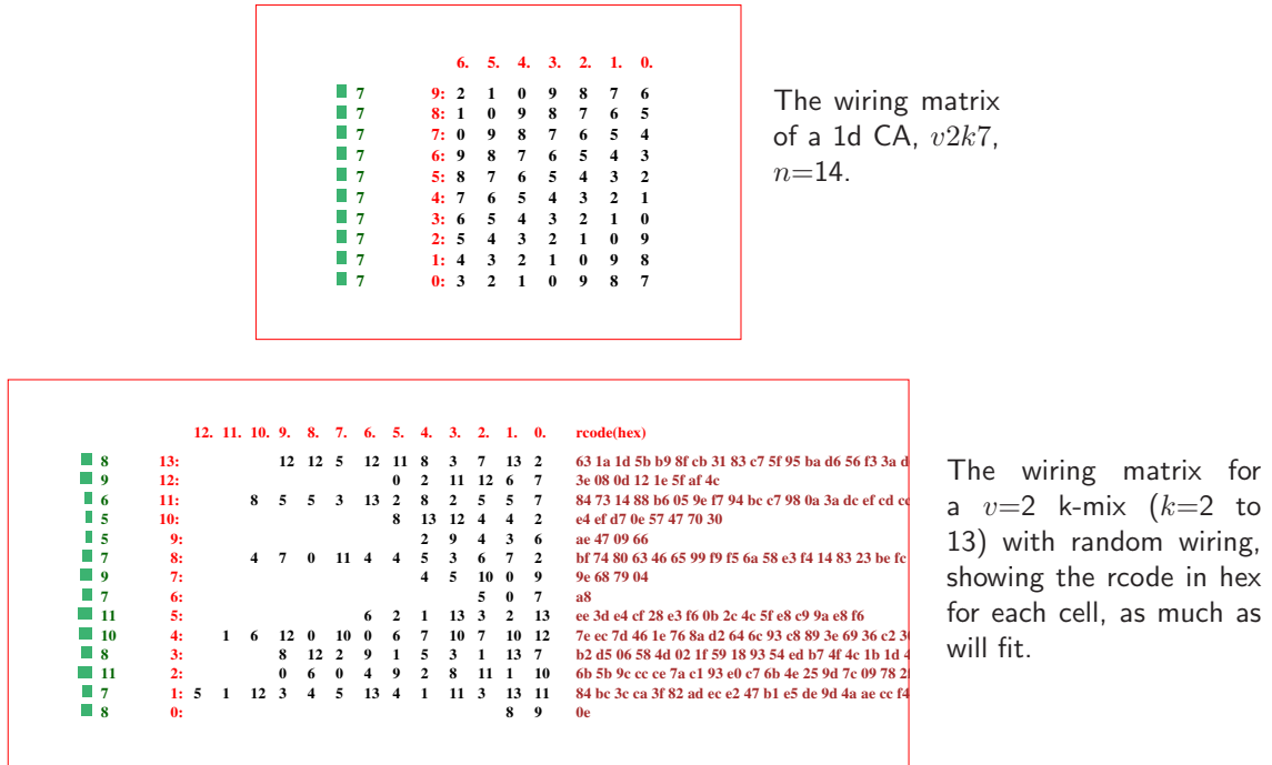
Figure 17.1: Wiring matrix examples. k-1, \dots, 0 indexes columns, n-1, \dots, 0 indexes rows. The column on the left shows the “out-degree” of each cell, the number of wires leaving it, also shown as a histogram. For a rulemix only (if set), rules are shown in hex, as much as will fit, in the right column. For k \leq 3 , decimal rules are added. If the matrix was set with m in section 17.1, the wiring can be set by hand as in a spread-sheet (section 12.6) and a rule in the active cell also appears in the rule window (section 16.19). If the matrix was set with M in section 17.1, the matrix cannot be amended, but there is an option to create a vector PostScript file, as in these figures.
