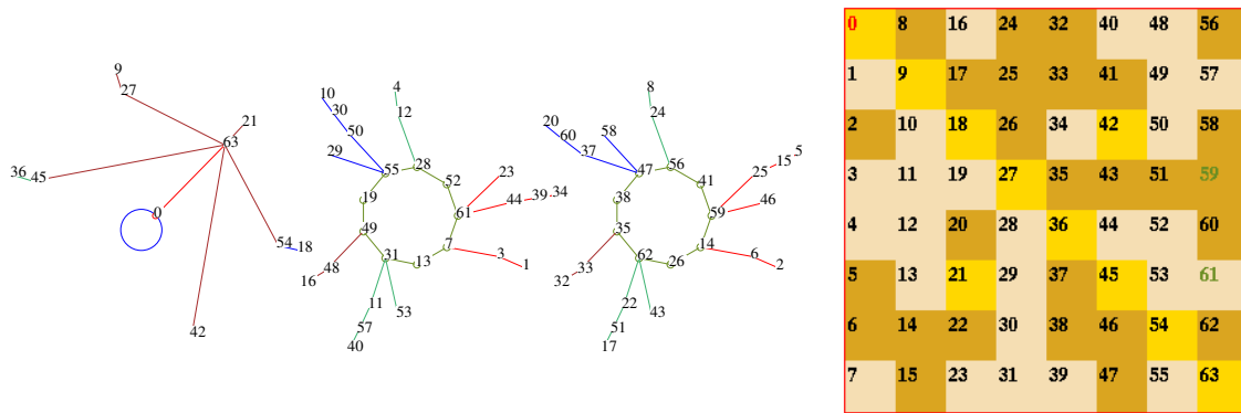
Figure 24.1: The state-space matrix of the basin of attraction field of a cellular automaton, v2k3 rcode (dec)110 , n=6 . Left : the uncompressed state transition graph. decimal numbers representing states. Right : The state-space matrix, where the 3 basins are represented by 3 colors. The decimal equivalents of states are shown in both cases.
