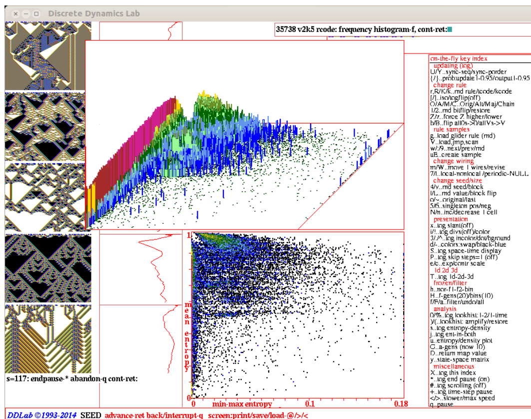
Figure 33.8: A snapshot of the DDLab screen after loading an automatic sample of 35738 rules, for 1d n=150 v2k5 isotropic CA, created in figure 33.7 (file v2k5iso1.sta). The sample was sorted by min-max entropy. Left : space-time pattern in blocks of 120 time-steps showing sequential examples, pausing at sample index 117 (section 33.7.2). Bottom Center : the scatter plot with min-max entropy. Top Center : the 2d histogram with the z -axis in log form.
