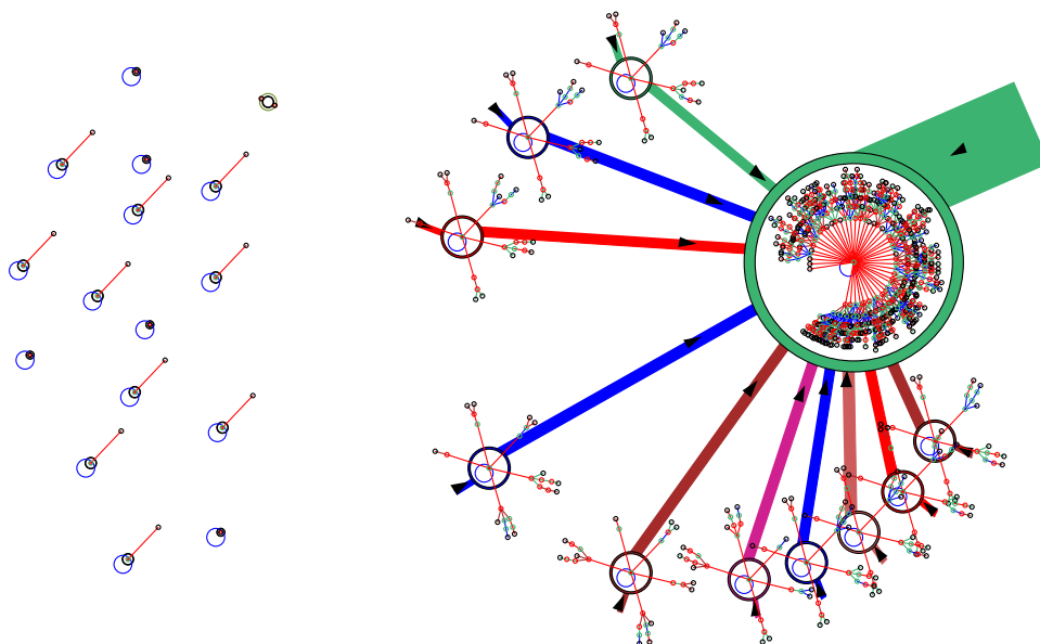
Figure 20.13: Disconnecting and isolating unreachable nodes. The isolated nodes are repositioned randomly on the far left side of the graph window. in this case with the default unreachableity threshold of zero. This example is for a jump-graph of a 1d CA, v2k3 rcode 104, n=10 . The basins of attraction were redrawn at the nodes (section 20.7).
