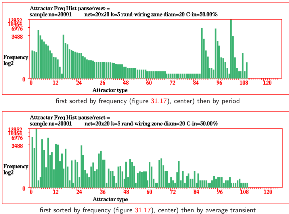
Figure 31.18: The attractor histogram for a sample of 30001 and 111 attractors, sorted by attractor period and average transient length, with log y -axis. (section 31.7.4).
