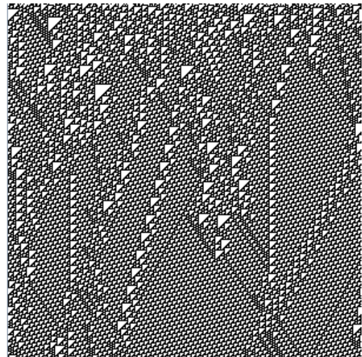
rule 110 (193 nr )
