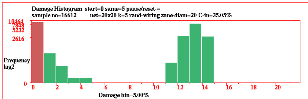
Figure 31.15: The damage histogram with the damage frequency allocated to 20 equal size bins, shown with the y axis in log form. This is a similar network as in figure 31.13, but with canalyzing inputs set to 35%, resulting in less ordered dynamics and a bimodal distribution of damage frequency.
