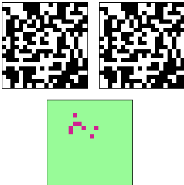
Figure 31.12: An example of 2d “damage”. The difference in dynamics between two 2d RBN. Above: the space-time patterns of two identical 20 \times 20 RBN (color by value), except that one bit was flipped in the initial state. The RBN has k=2 , with connections as in figure 31.6.1. Below: the “damage spread” between the two, which has stabilized after a number of time-steps, shown as a third space-time pattern. In this example keep-f was selected in section 31.6, so that once a cell is “damaged” - it stays “damaged”.
